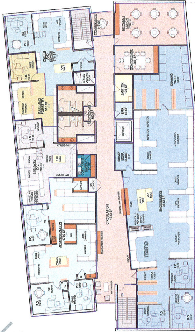
1 02 Second Floor 1/8" = 1'-0"
