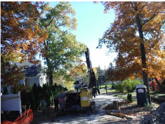
Drill rig probing for ledge Rockwood Lane 10/27/15
